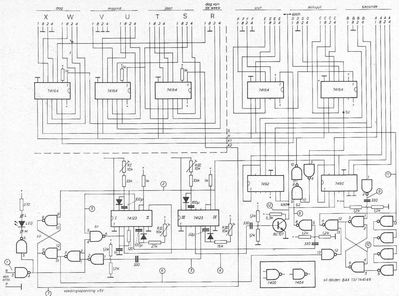
Fig. 10. Decodeerschakeling.
